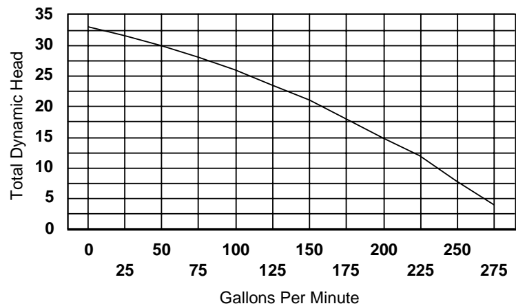
Piranha Agitator Pump Severe Duty Model P-3-A
