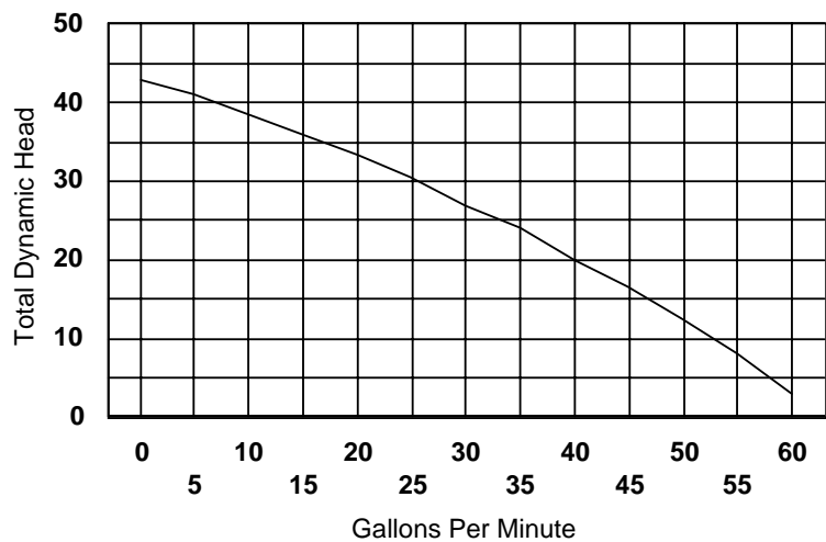
Piranha Agitator Pump Model PS-75-A/AJ
