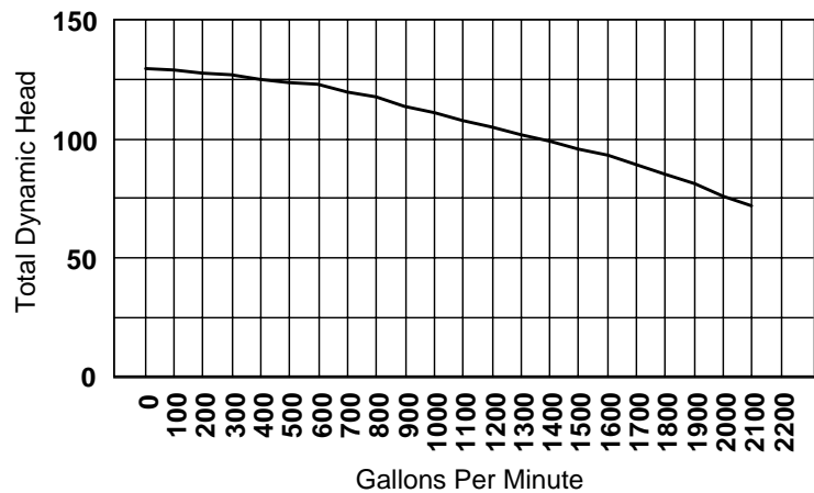
Piranha Agitator Pump Severe Duty Model P-75-A
