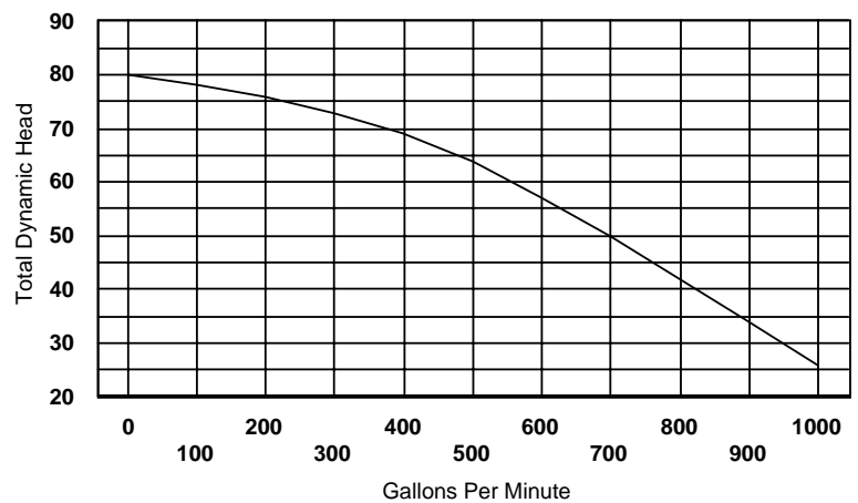
Piranha Agitator/Slurry Pump Model PS-2000-A
